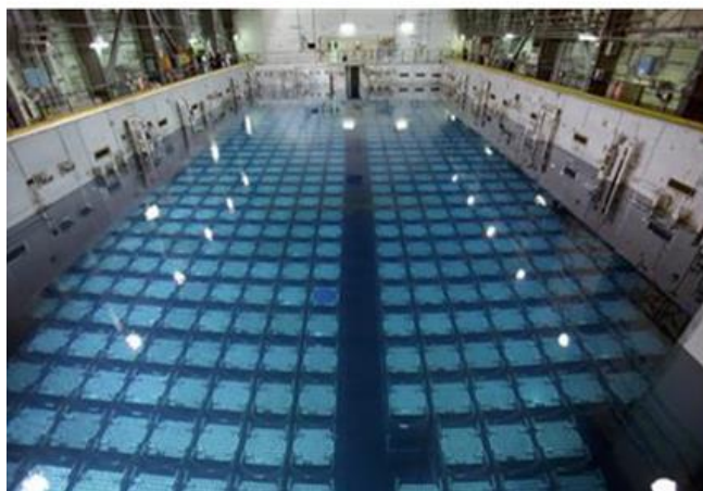
Spent fuel bundles stored in a nuclear plant.
