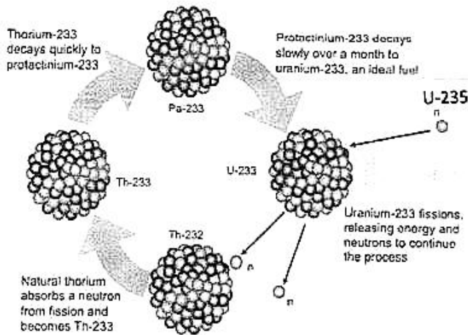
Neutron-induced breeding of thorium to fissile uranium
