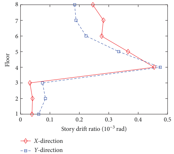
FIGURE 10: The story drift ratio curves of the structure by the pushover analysis.
