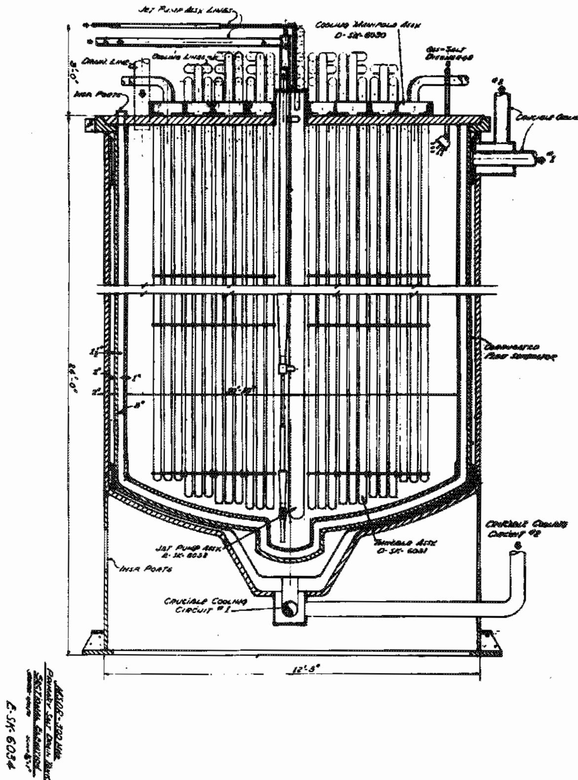
Fig. 8.5. MSDR - 300 MW(e) primary salt drain tank sectional elevation.
