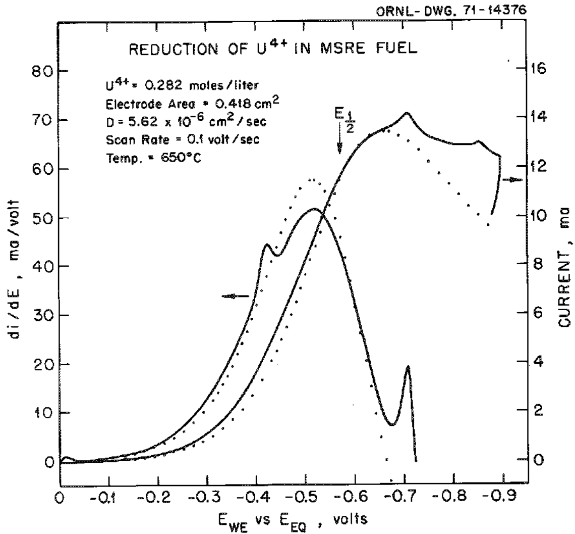
Fig. 5.12. Current-voltage wave and derivative for reduction of U^{4+} to U^{3+} theoretical points (.), experimental curve (-).
