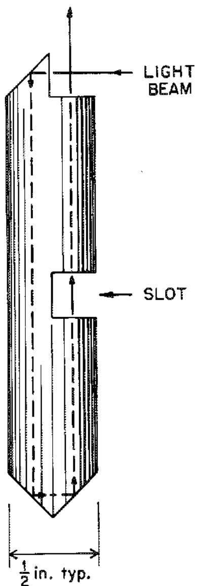
Fig. 5.16. Slotted optical probe for spectral analysis.
