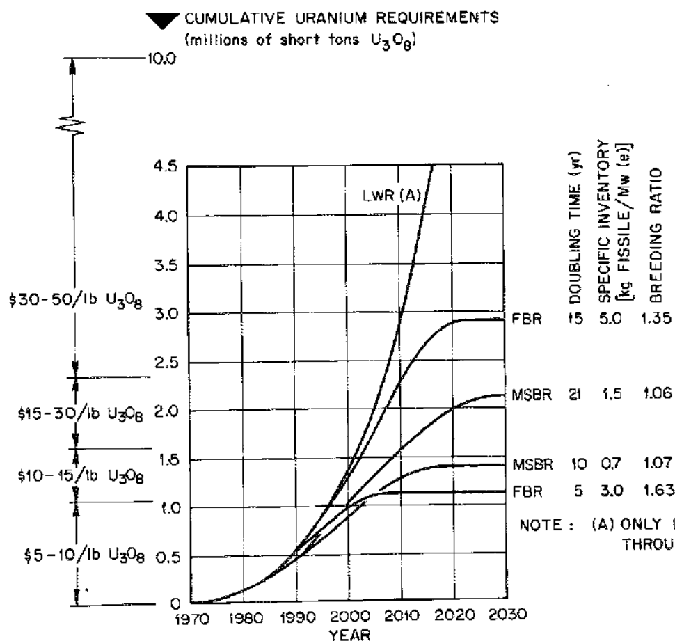
Fig. 4.1. Effect of breeders on the ore requirements of the U.S. nuclear power economy if breeders are introduced in the mid-1980's and only breeders are built after 1998.
