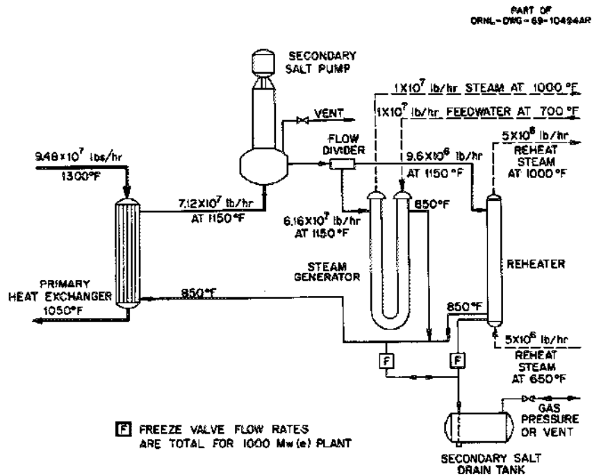
Fig. 8.3. Secondary salt and steam system molten salt breeder reactor flow diagram-1000 MW(e) Unit-Mark II.
