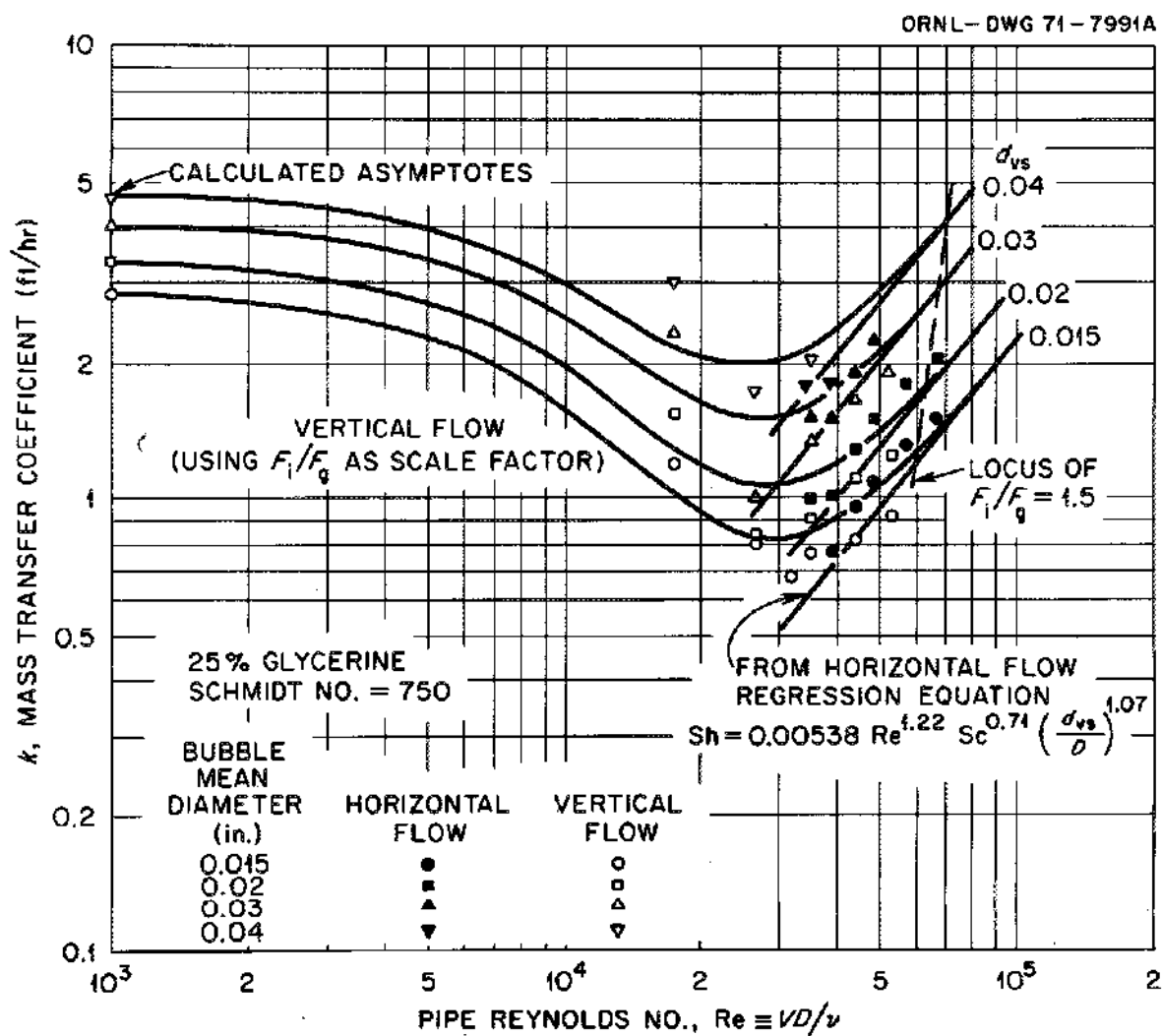
Fig. 8.13. Typical mass transfer coefficients obtained for stripping oxygen from aqueous glycerine solutions.
