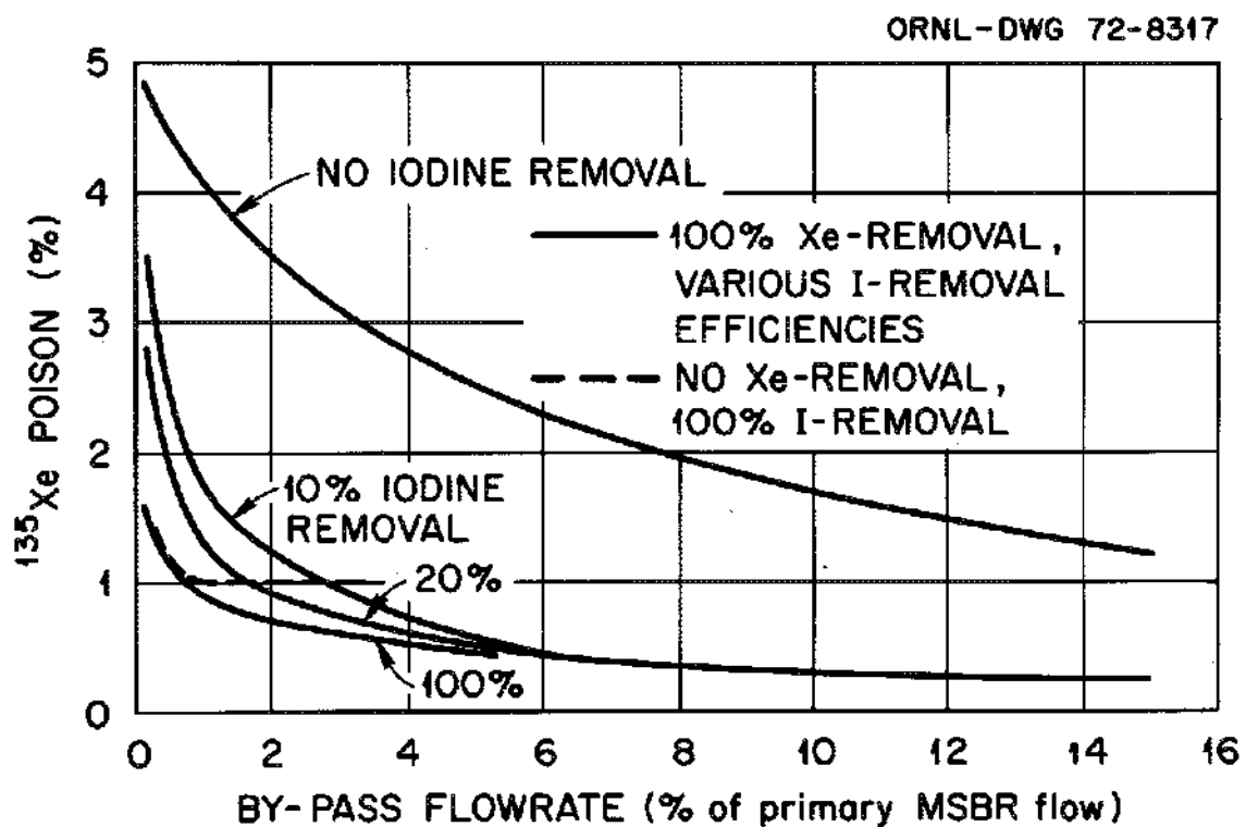
Fig. 8.10. Xenon-135 poison fractions using combined xenon and iodine stripper with uncoated graphite.
