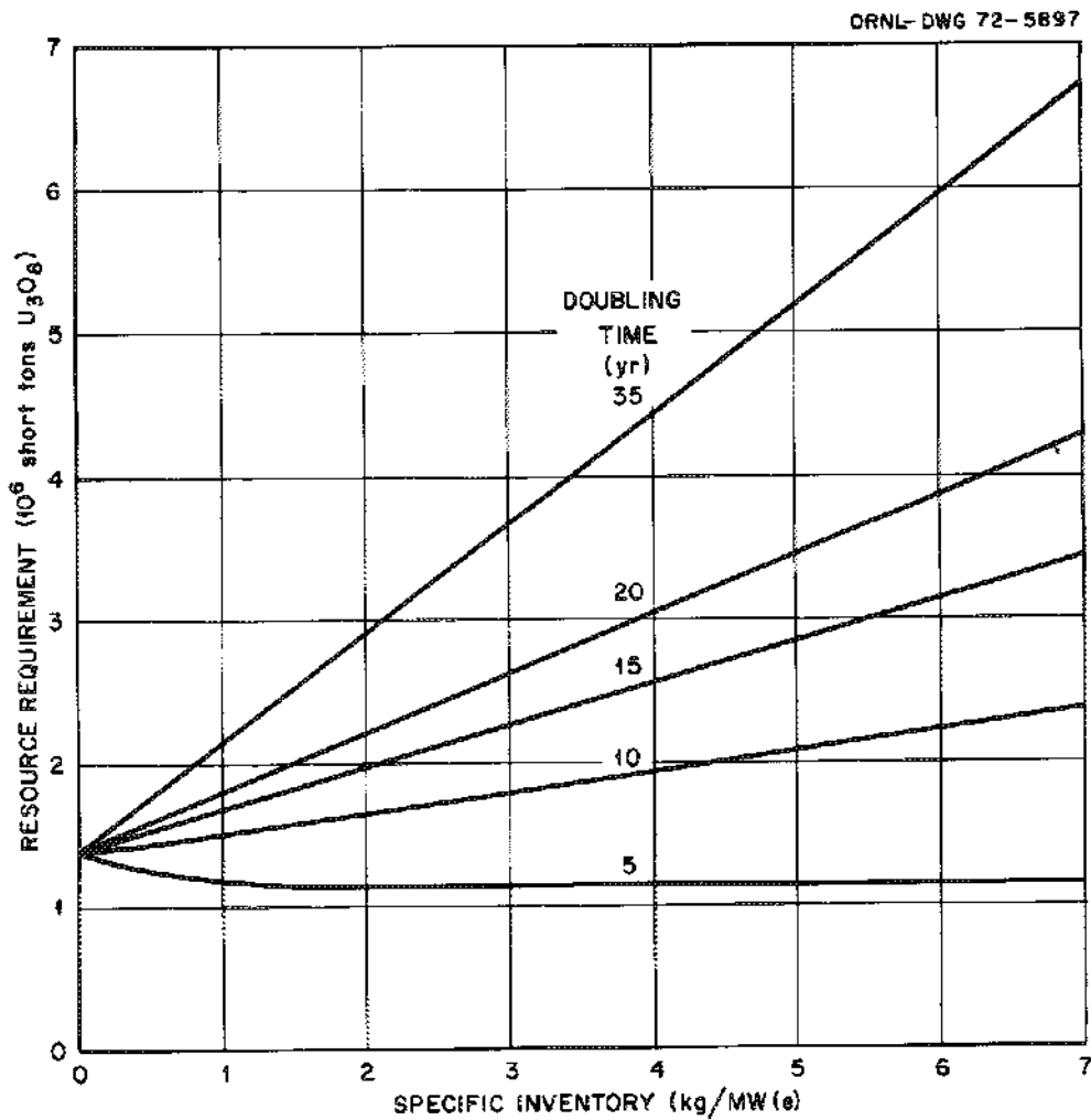
Fig. 1.3. The effect of the fuel utilization characteristics of breeders on the cumulative uranium ore requirements for a growing U.S. nuclear power economy.
