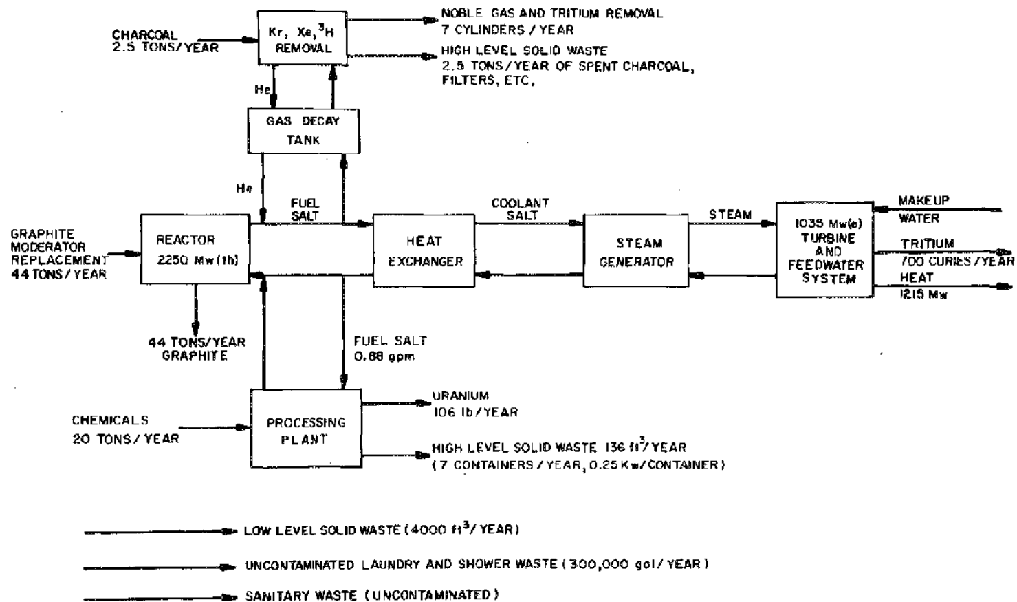
Fig. 14.2. Materials flow diagram for a 1000-MW(e) MSBR unit.
