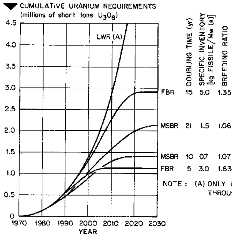
Fig. 1.2. Effect of breeders on the ore requirements of the U.S. nuclear power economy if breeders are introduced in the mid-1980's and only breeders are built after 1998.
