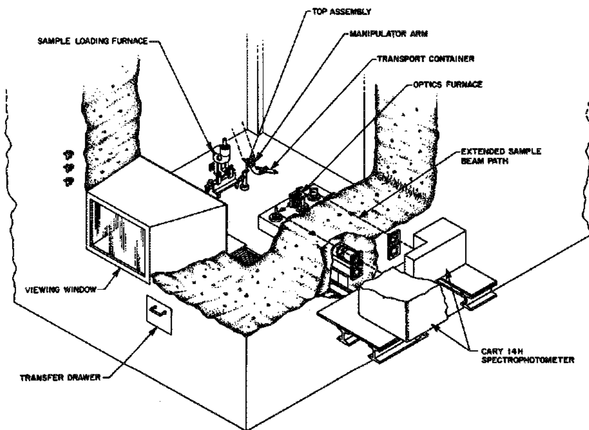
Fig. 5.11. Spectrophotometer installation.
