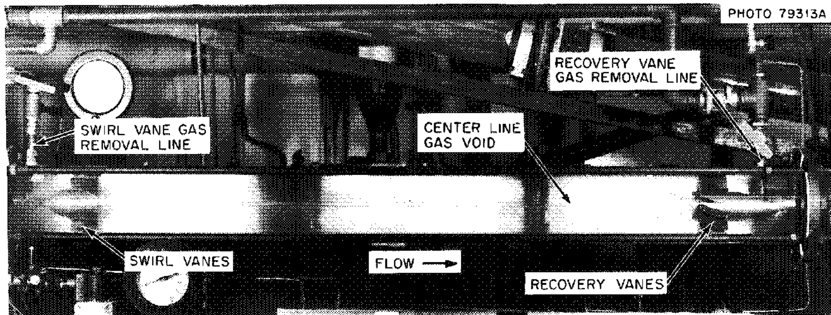
Fig. 8.14. MSRE inline gas separator mockup.
