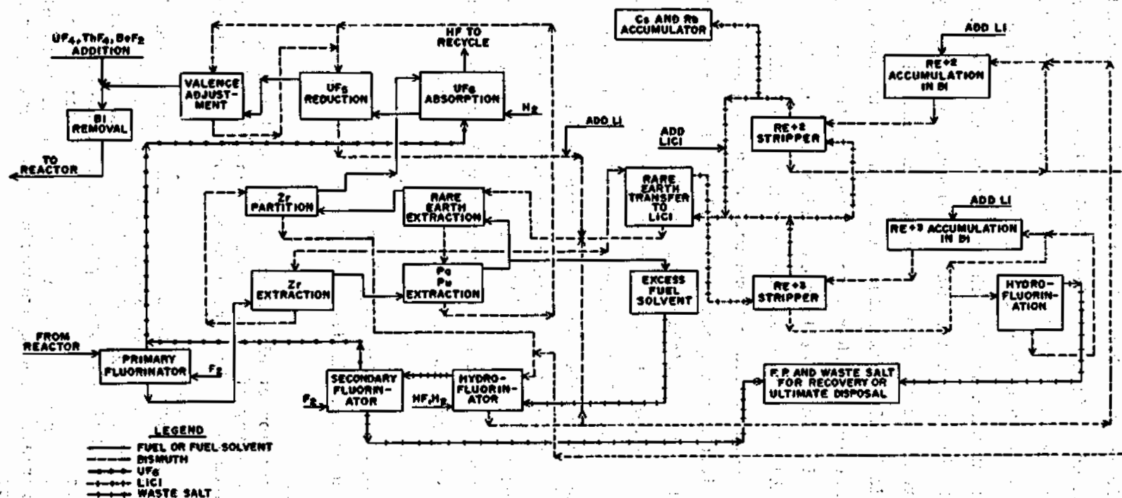
Fig. 8. Preliminary flowsheet for fuel reprocessing plant in a denatured MSR.
