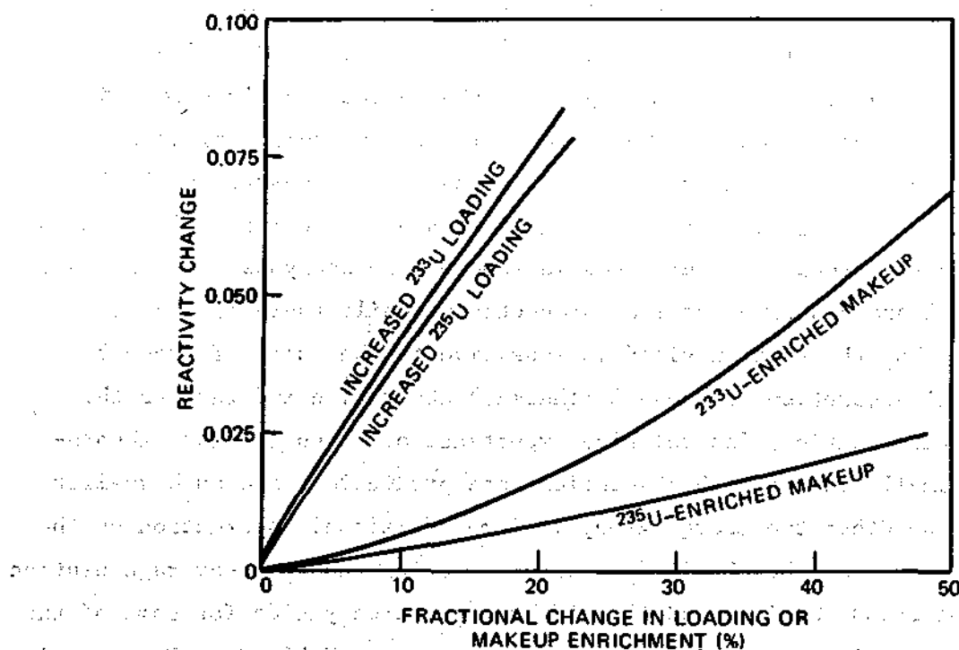
Fig. 6. Effect of initial loading and enriched makeup on equilibrium reactivity.
